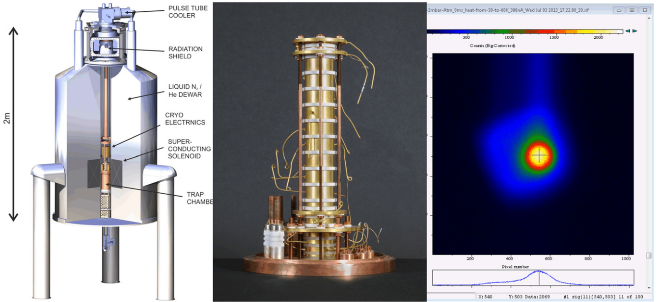
Figure 4. Schematic view of the superconducting magnet setup, the Penning trap used for spectroscopy, and a CCD image looking into the trap during ion production.
