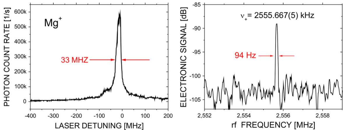
Figure 2. Axial optical laser cooling signal of confined \text{Mg}^+ ions in SPECTRAP (left) indicating an ion temperature of around 60 mK, and radial electronic detection signal of confined \text{Mg}^+ ions (right).
