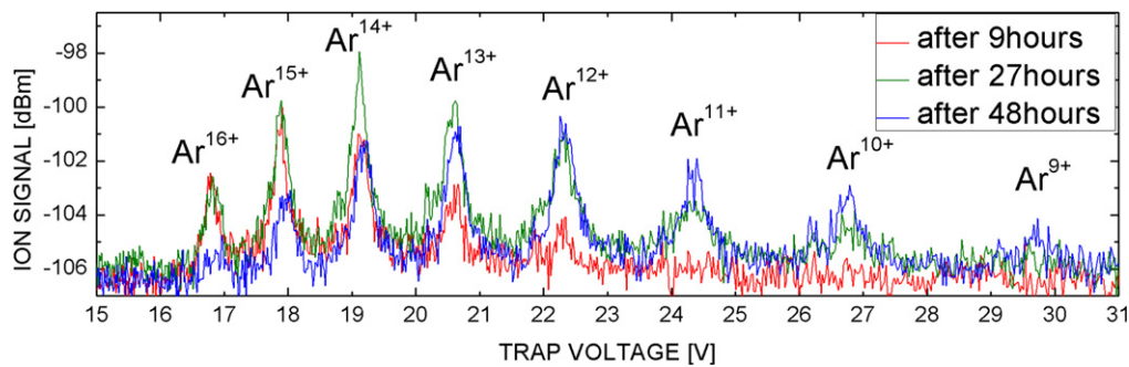
Figure 5. Ion charge state spectrum of the same ion cloud at different times after in-trap ion creation.
