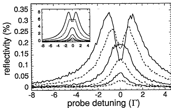
FIG. 3. Bragg reflectivity as a function of probe laser detuning for densities from 3 \times 10^9 to 8 \times 10^{10} \text{ cm}^{-3} , increasing by roughly a factor of 2 between traces. For increasing densities, the spectra become broader and develop a dip at resonance. The temperature of the atoms is T = 12 \mu\text{K} and the initial localization is \sim \lambda/7 . The inset (same axes) shows calculated reflection spectra for the same parameters in a one-dimensional model, neglecting some experimental details such as the shape of the sample, the probe beam profile, and the probe divergence.
